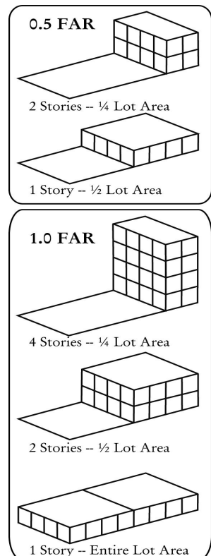
FIGURE 24-302-2 FLOOR AREA RATIO
